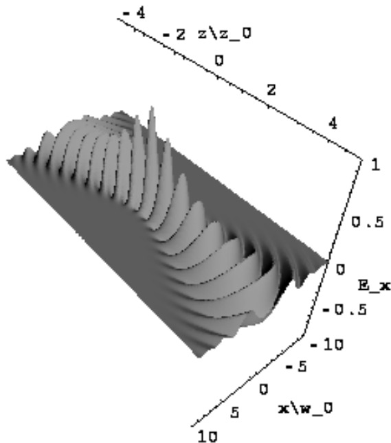
Figure 1: The electric field E_x(x, 0, z) of a linearly polarized Gaussian beam with diffraction angle \theta_0 = 0.45 , according to eq. (67).
