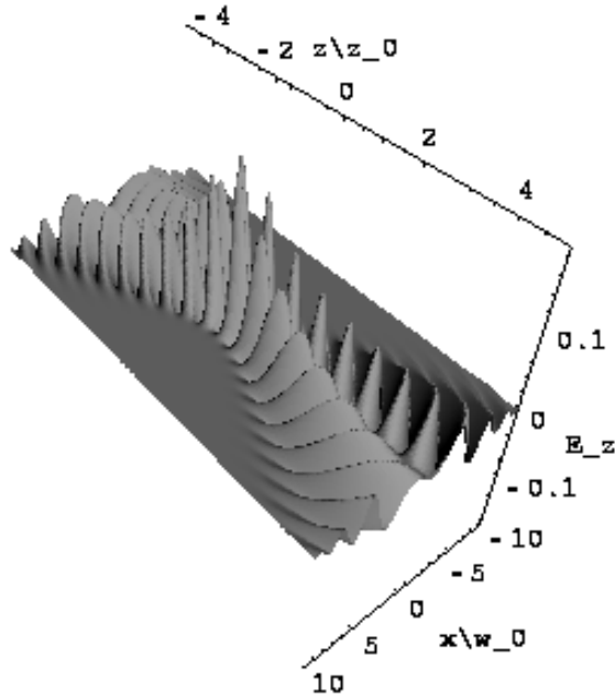
Figure 2: The electric field E_z(x, 0, z) of a linearly polarized Gaussian beam with diffraction angle \theta_0 = 0.45 , according to eq. (67).
